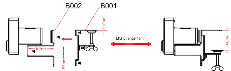
B002 Application diagram
